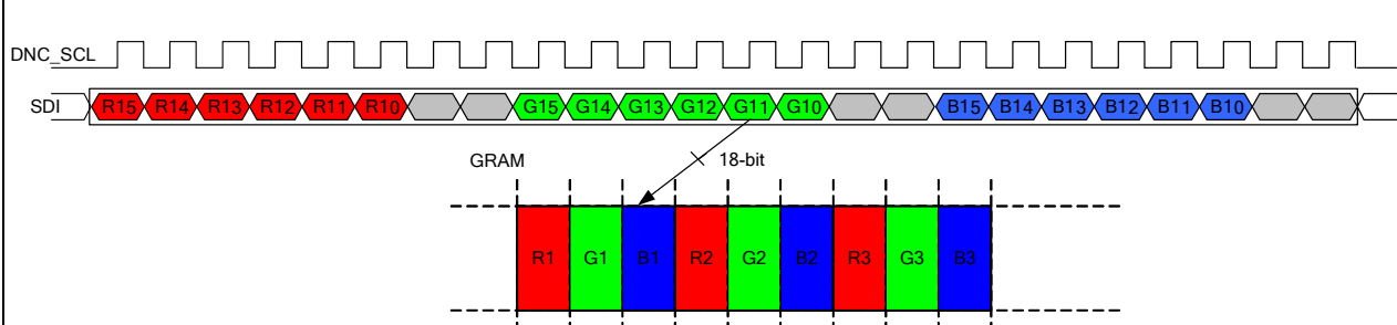
Figure 5.32 Data write timing in 4-wire serial bus system interface
