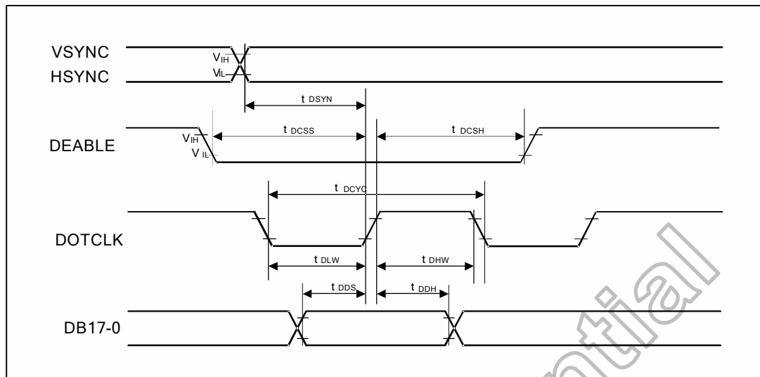
Figure 11.5 RGB interface characteristics
