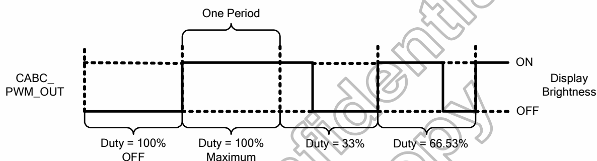
Figure 7.20 CABC_PWM_OUT output duty
